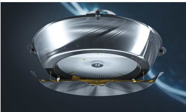
The particles collide with the rotating plate and are thrown toward the sides of the filter housing.
